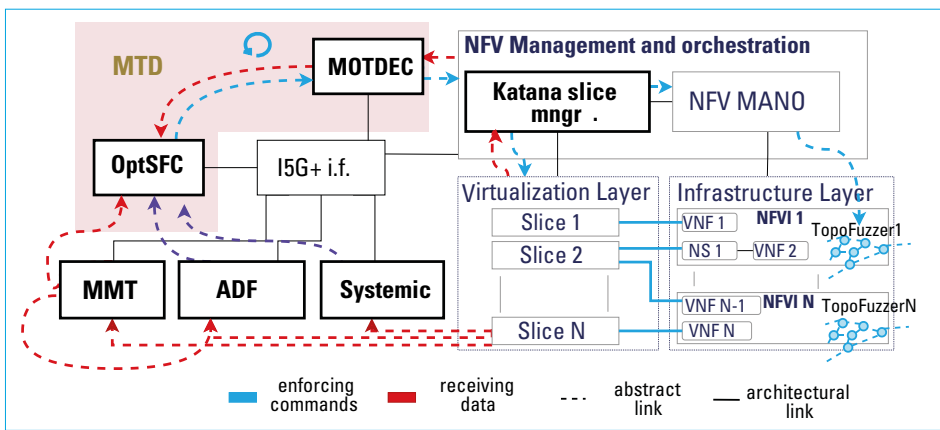
Fig. 14. Demo 3 architecture
